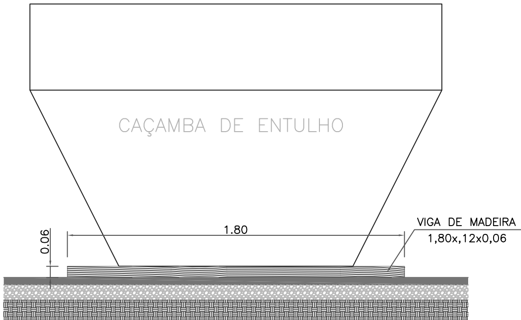
VISTA FRONTAL
